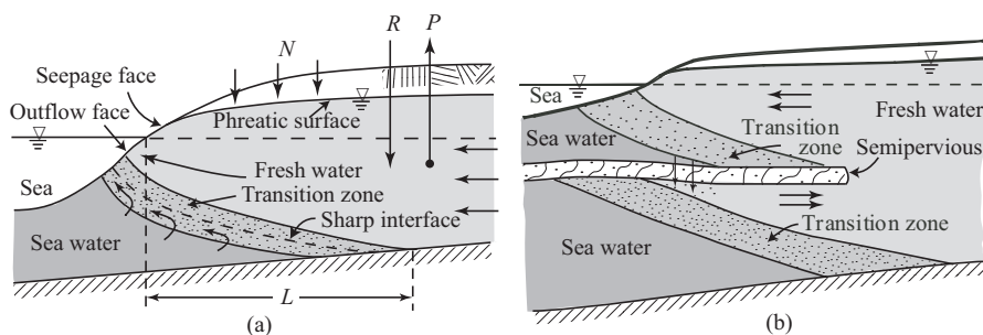
Figure 9.1.2: Typical cross-sections of transition zones in coastal aquifers.
