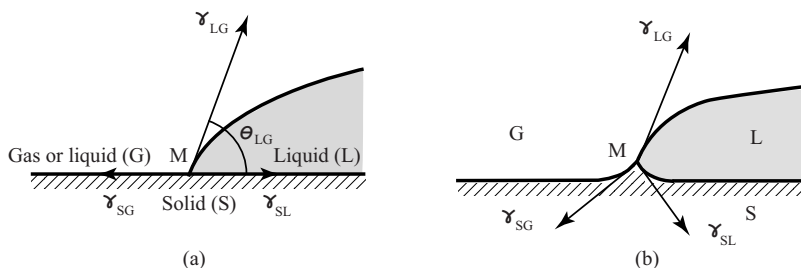
Figure 6.1.1: Interfacial tension.
