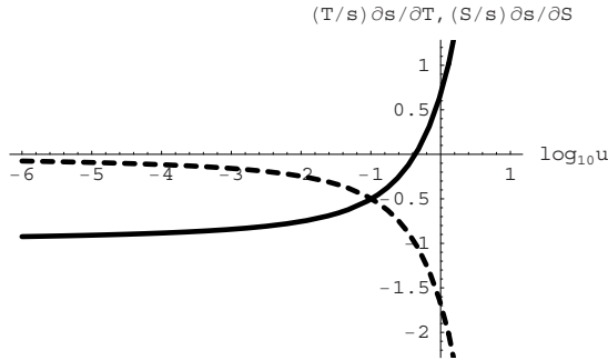
Figure 10.2.3: Normalized sensitivity coefficient for a pumping well in a confined aquifer. Solid line: C_T ; dash line: C_S .
