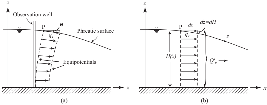
Figure 4.5.2: Dupuit assumption.
