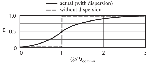
Figure 7.1.2: Breakthrough curve in one-dimensional flow in a column of homogeneous porous material; \varepsilon \equiv (c(t) - c_o)/(c_1 - c_o)
