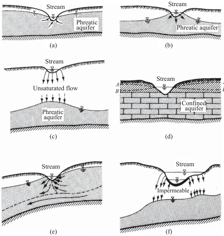
Figure 3.5.1: River-aquifer relationships. (a) Effluent stream. Groundwater drains into stream. (b) Influent stream. River contributes to groundwater flow. (c) Influent stream (deep water table). River contributes to groundwater. (d) Influent stream (piezometric surface B), or effluent one (piezometric surface A) intersecting a confined aquifer. (e) A stream which is both influent and effluent. (f) A partly clogged influent stream.
