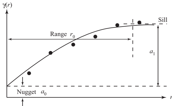
Figure 10.2.1: Empirical semivariogram constructed from data.
