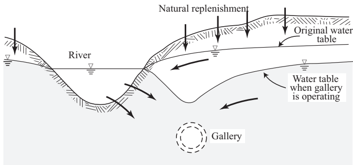
Figure 3.4.5: Induced recharge.
