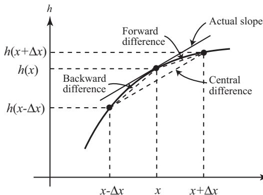
Figure 8.1.2: Geometrical interpretation of the forward, backward and central difference approximations of the derivative of a function.
