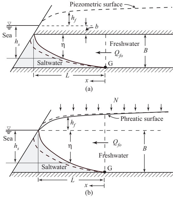
Figure 9.2.7: Stationary interface derived by the Dupuit (Ghyben-Herzberg) approximation.
